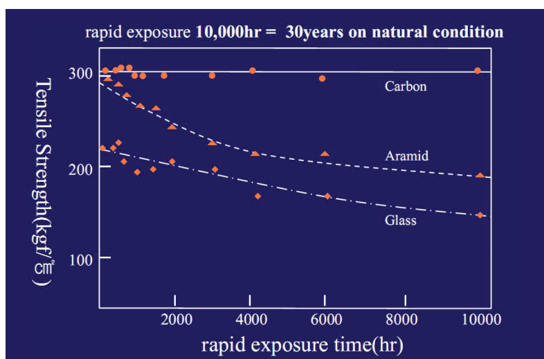
Fig 10. Graphs showing deterioration with time in rapid exposure test.
