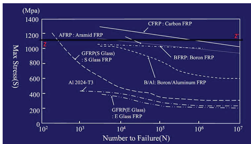
Fig 11. Graph showing fatigue characteristics of different fibres.
