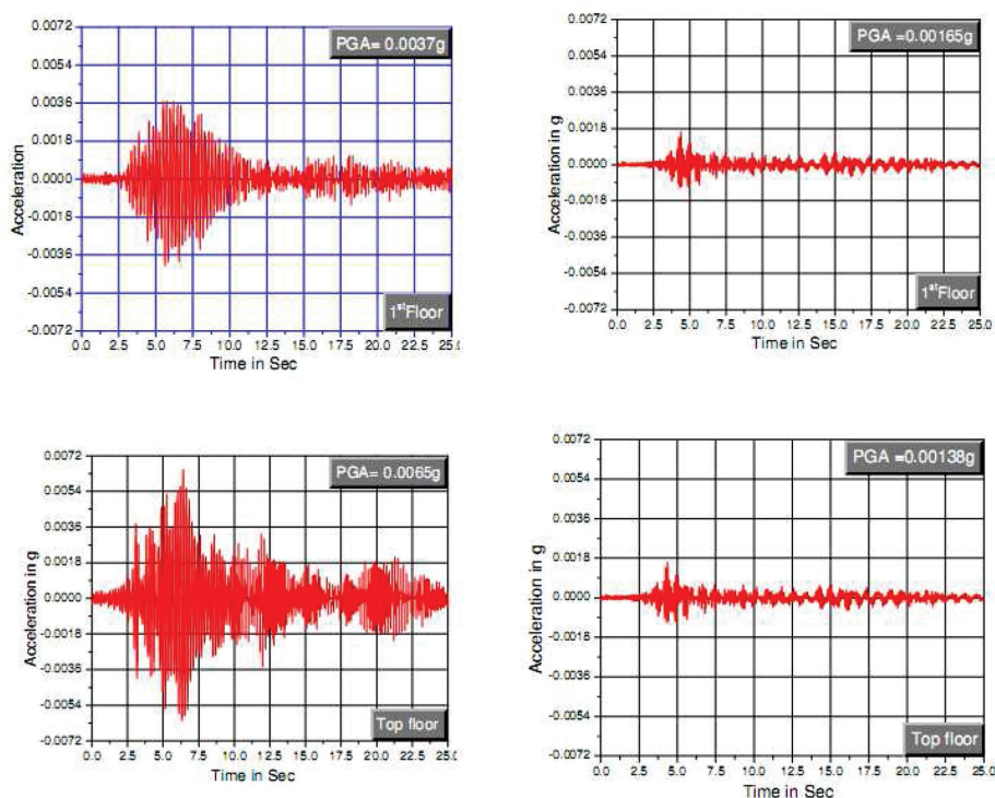
Fig 16 Response of Buildings subjected to actual earthquakes MAGNITUDE: 5.2, Nov 06, 2006, LOCATION: 24.736o N 95.223o E, DEPTH: 122.6 km
