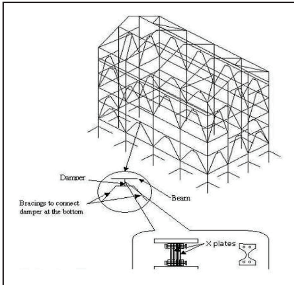
Fig 12 Location of Dampers
