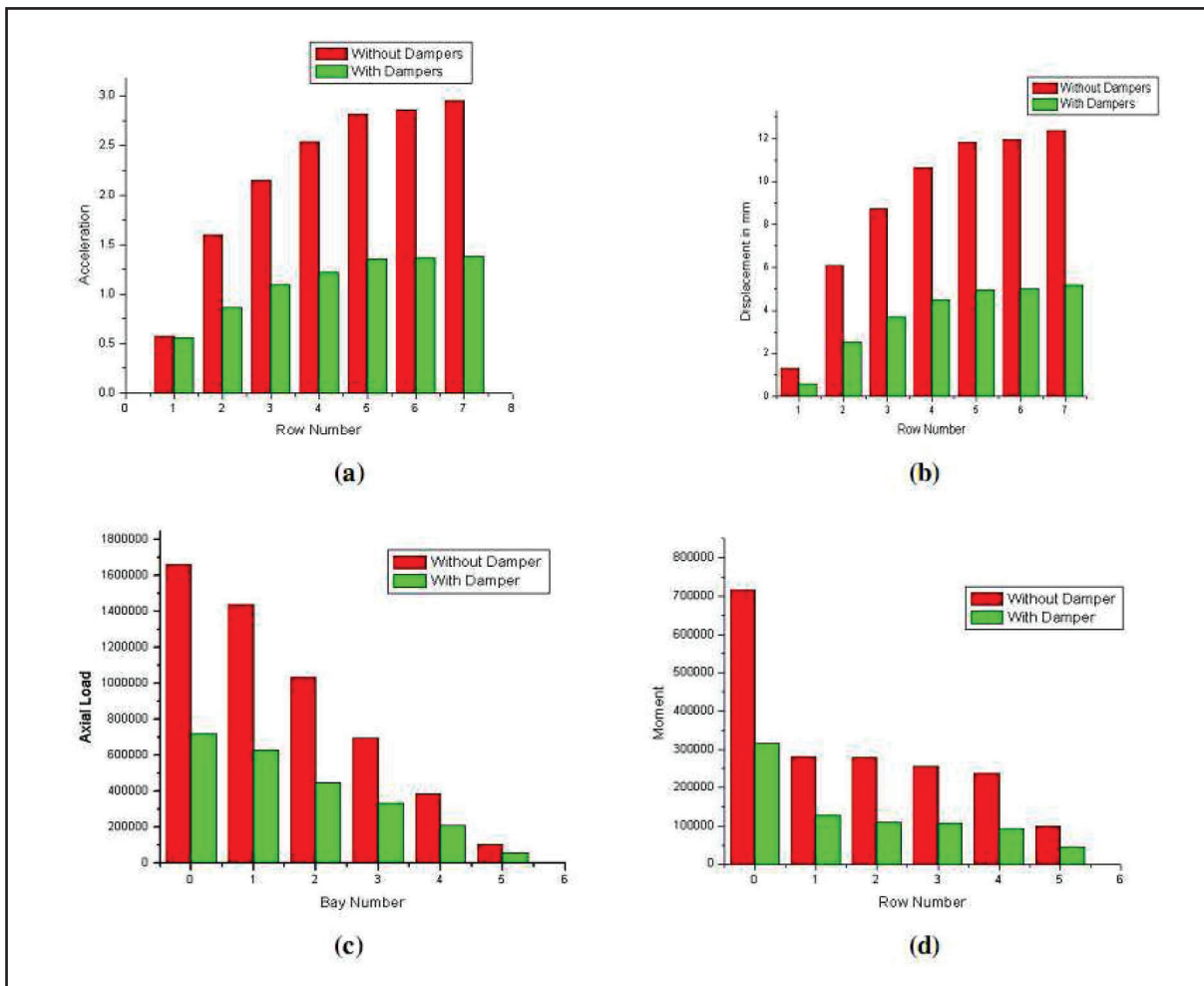
Fig 14 Comparative Plots of Seismic Analysis.
