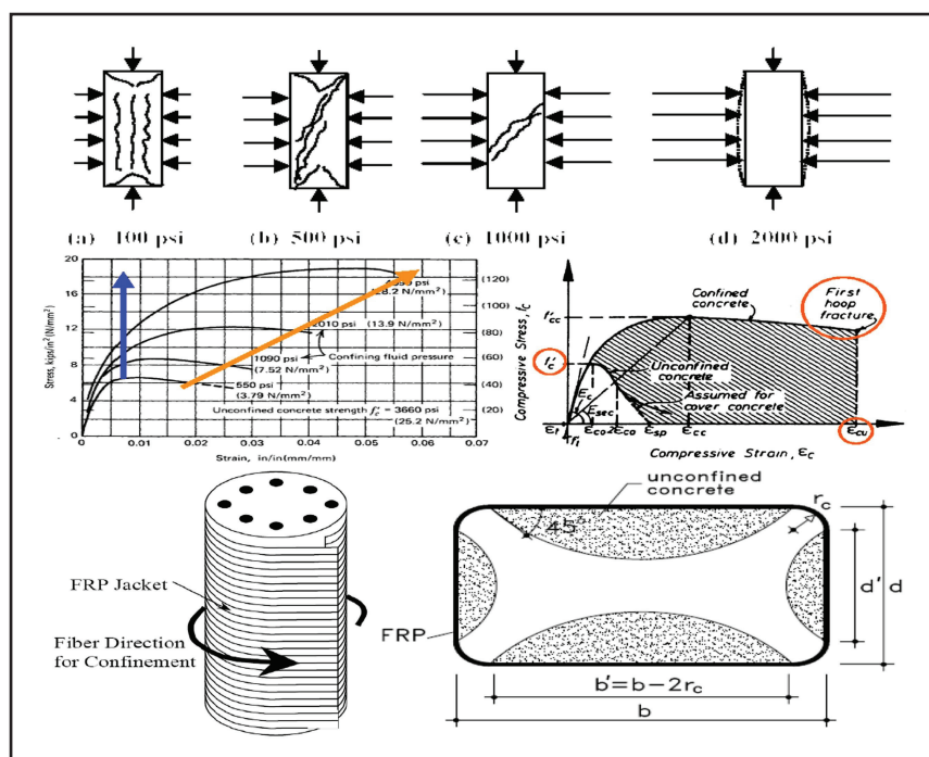
Fig 7 the Concept of Confinement
