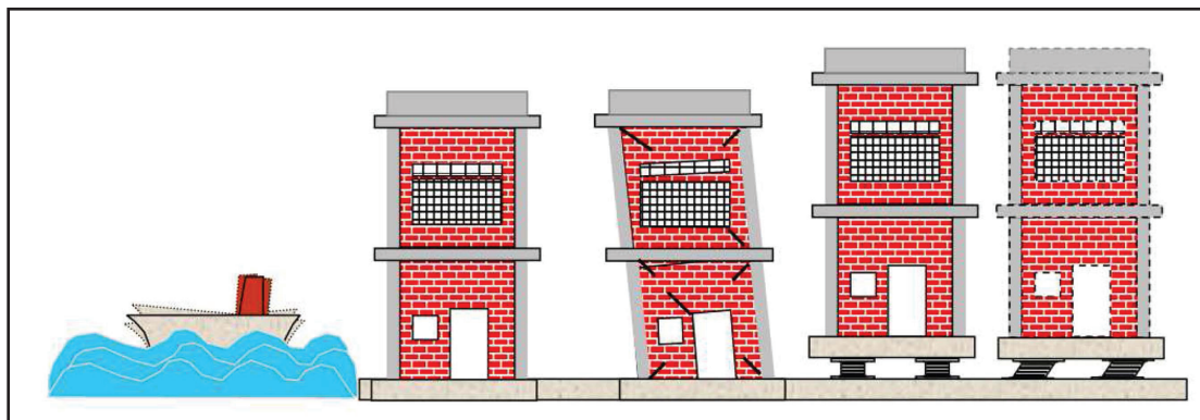
Fig 4. Principles of Base Isolation Technology
