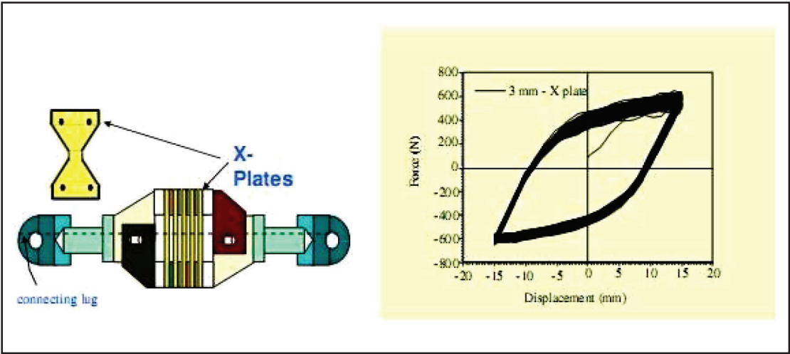
Fig 1 Elasto- Plastic damper and the hysteretic Charecteristic of the x-plate
