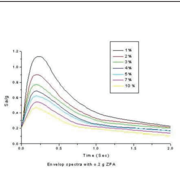
Fig 13 Response Spectrum
