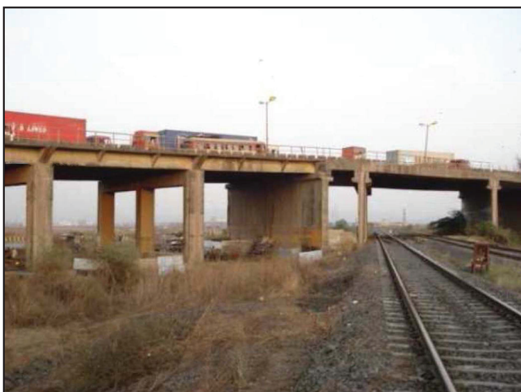
Figure 3: Rail Over Bridge (ROB) at Karal junction of JNPT 5
