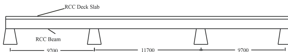
Fig. 1 Support arrangement for Girders.
