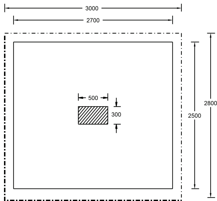
Fig. 7 Load dispersion and critical section for punching shear in slab.
