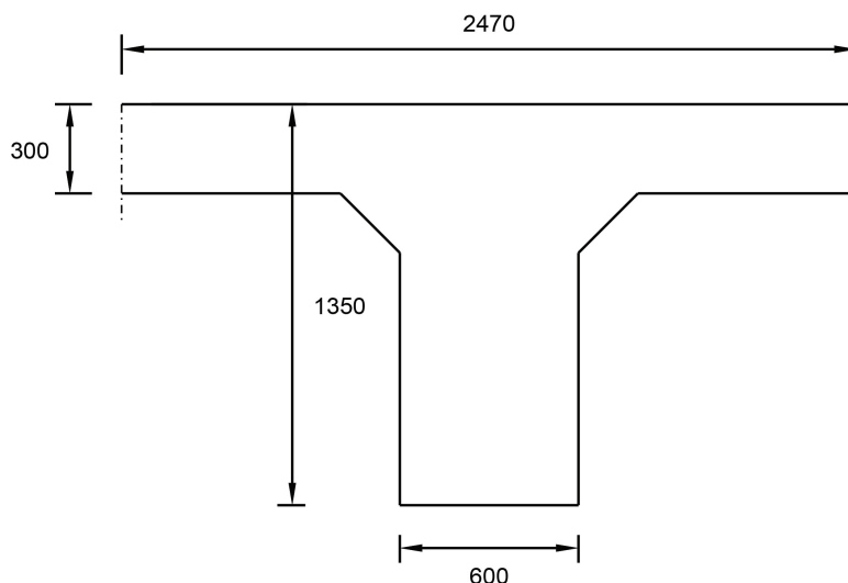
Fig. 2 Typical Cross-Section of T- Beams.
