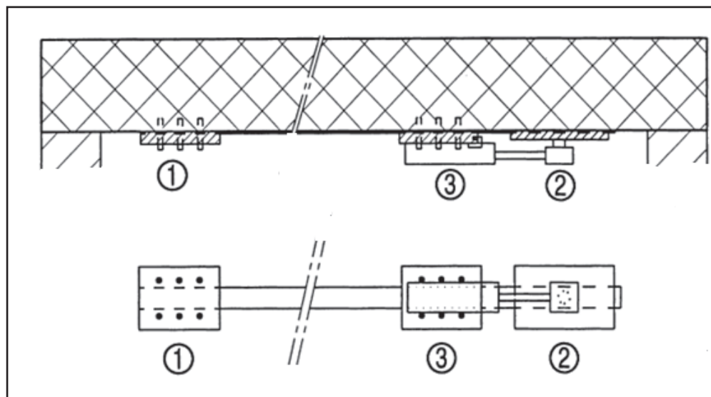
Fig-2 Pre-stressing System 1) fixed anchor 2) mobile anchor 3)pre-stressing system
