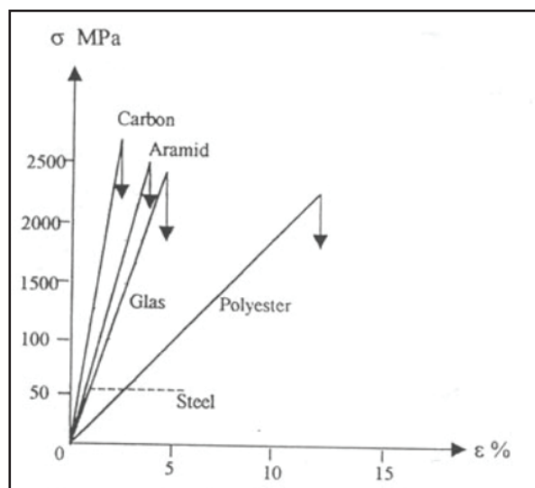
Fig 1. The comparative strength of different materials
