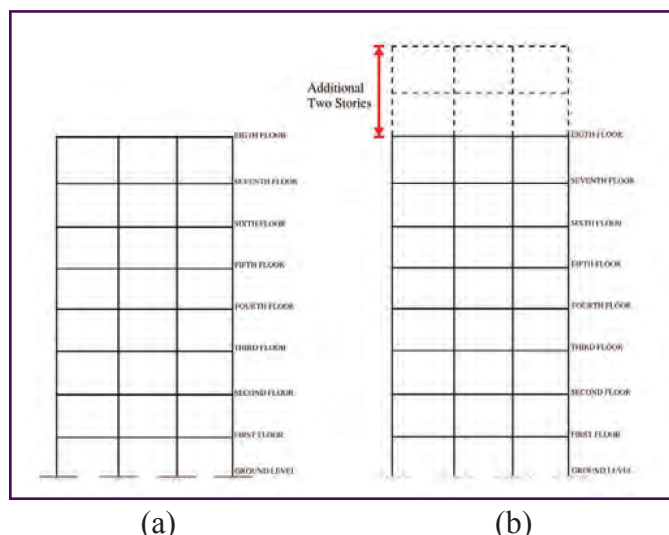
(a) Existing G+8 Storey Building
